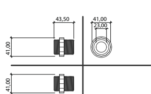
NIPPLE 1"
