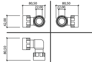
ELBOW FxM 1"
