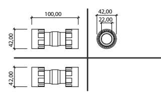
NIPPLE 1" x 3/4"
